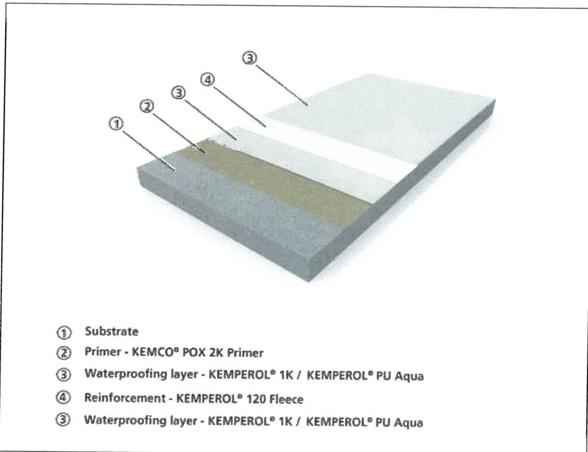
Classification of the roof waterproofing system “KEMPEROL® 1K / KEMPEROL® PU Aqua”
